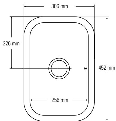
Top view * overflow
