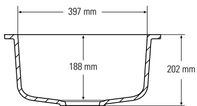
Side cross-section
