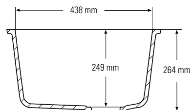
Side cross-section
