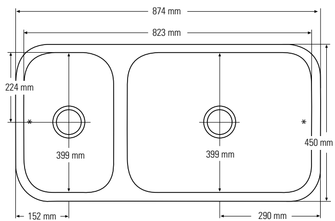
Top view * overflow
