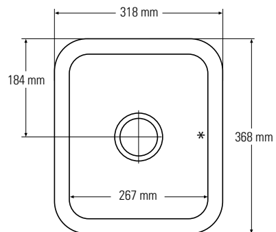
Top view * overflow
