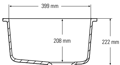
Side cross-section
