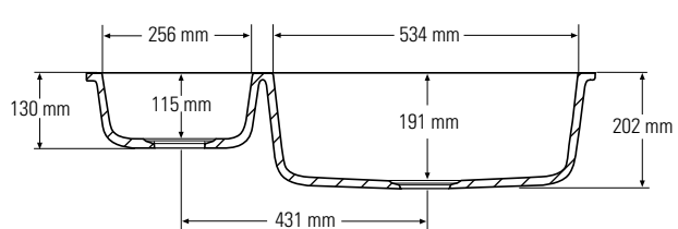
Front cross-section
