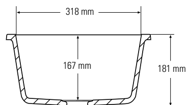
Side cross-section
